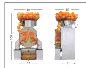
Citrocasa 8000 XB with Juice-Tank Art.-No. 80.002
